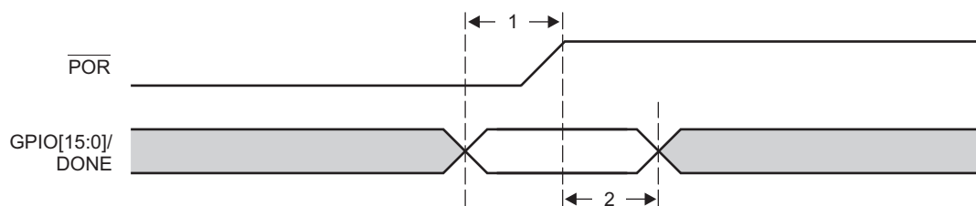
Figure 7-16 Boot Configuration Timing
