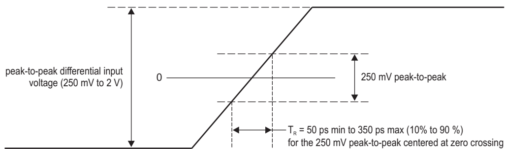
Figure 7-30 PLL Transition Time
