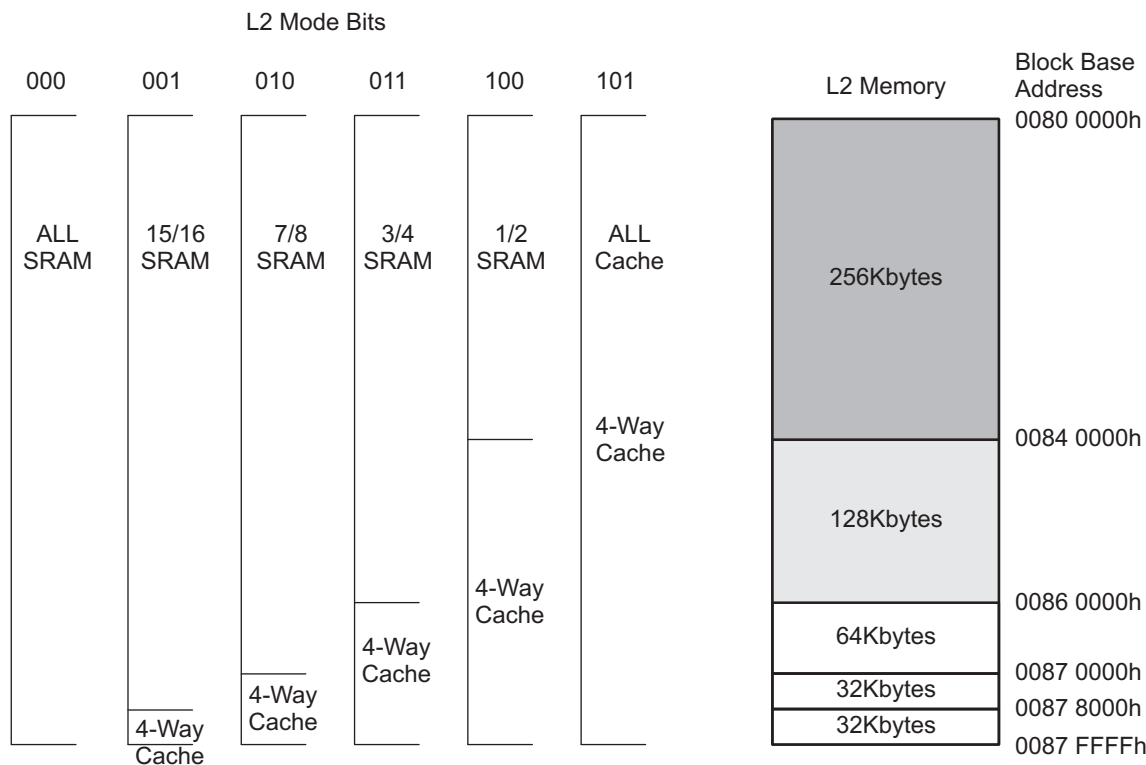
Figure 5-4 TMS320C6671 L2 Memory Configurations
