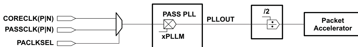
Figure 7-34 PASS PLL Block Diagram
