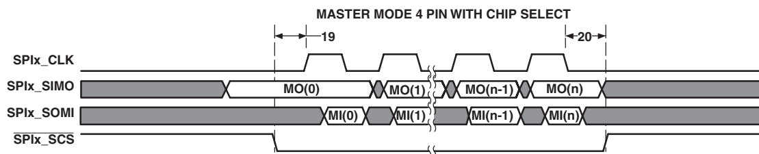
Figure 7-41 SPI Additional Timings for 4 Pin Master Mode with Chip Select Option
