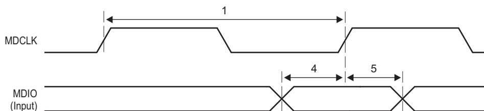
Figure 7-51 MDIO Input Timing
