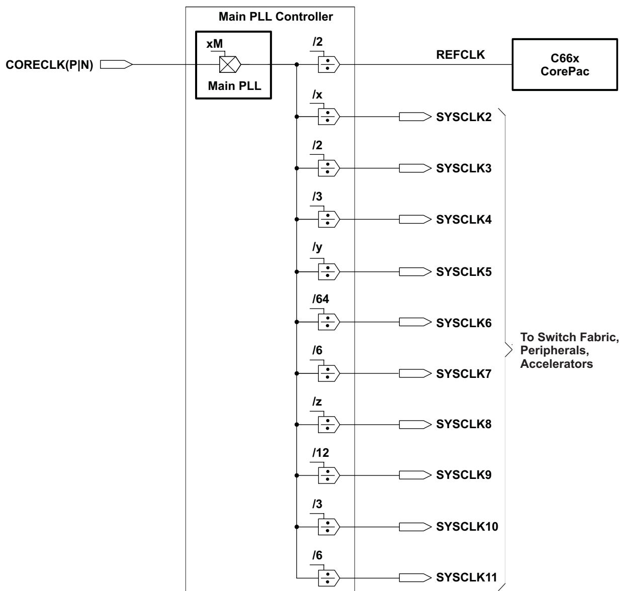
Figure 7-17 Main PLL and PLL Controller
