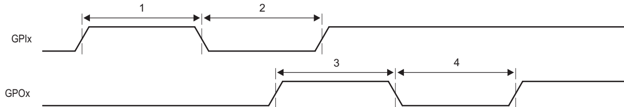
Figure 7-54 GPIO Timing
