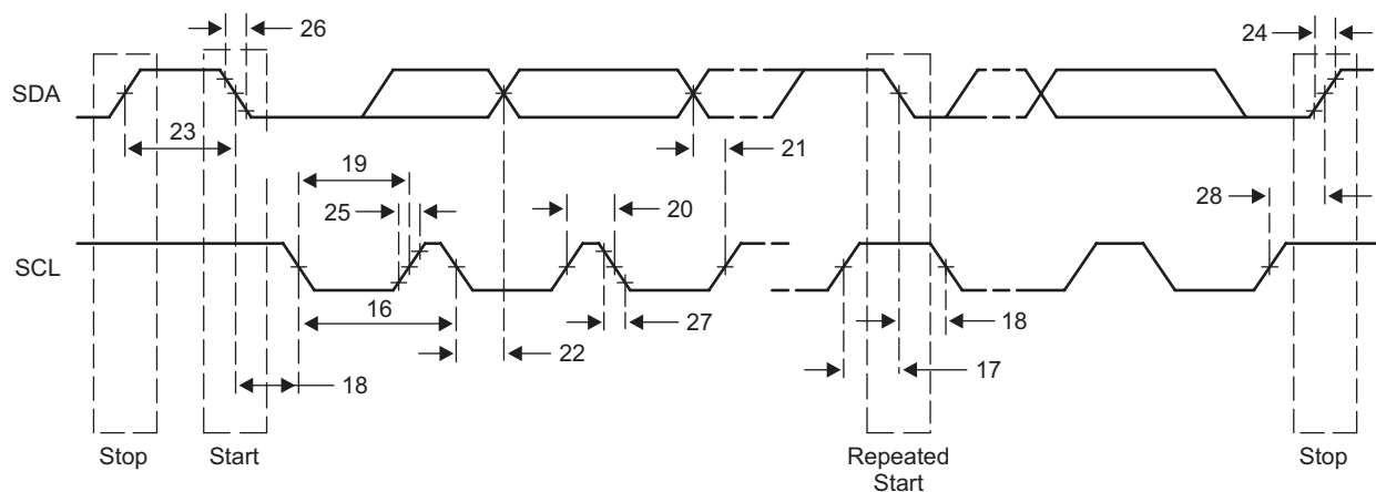
Figure 7-39 I 2 C Transmit Timings
