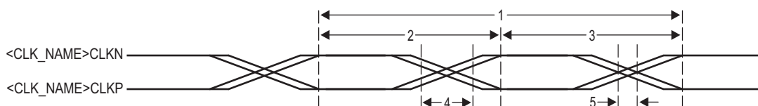
Figure 7-29 Main PLL Controller/SRIO/HyperLink/PCIe Clock Input Timing
