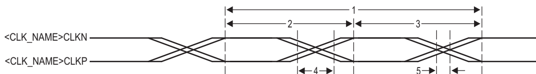
Figure 7-36 PASS PLL Timing
