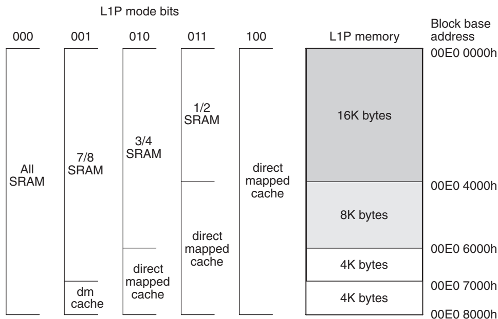
Figure 5-2 TMS320C6671 L1P Memory Configurations
