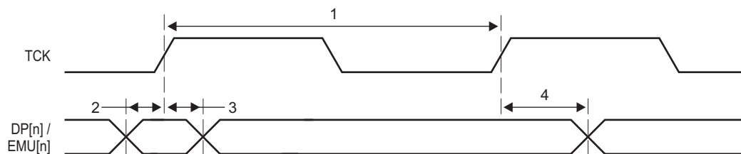
Figure 7-57 HS-RTDX Timing
