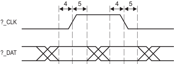
Figure 7-44 HyperLink Station Management Receive Timing
