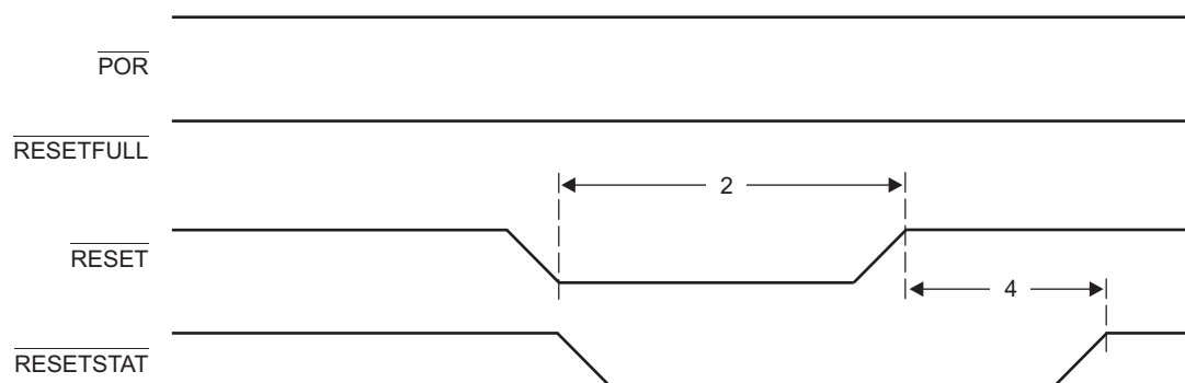
Figure 7-15 Soft/Hard-Reset Timing
