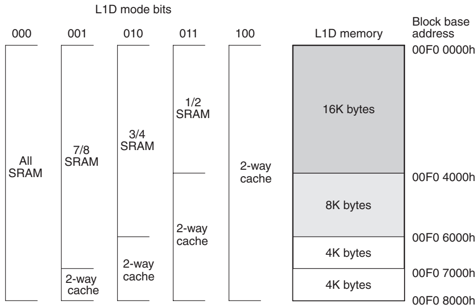
Figure 5-3 TMS320C6671 L1D Memory Configurations
