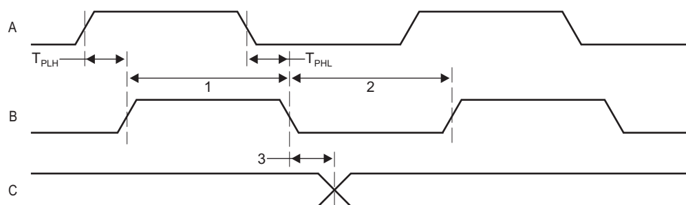
Figure 7-55 Trace Timing
