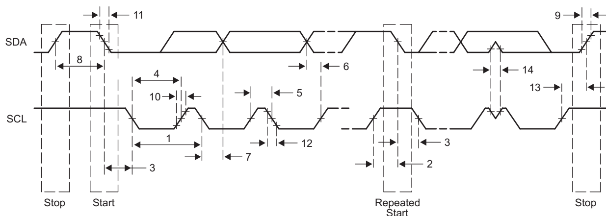
Figure 7-38 I 2 C Receive Timings
