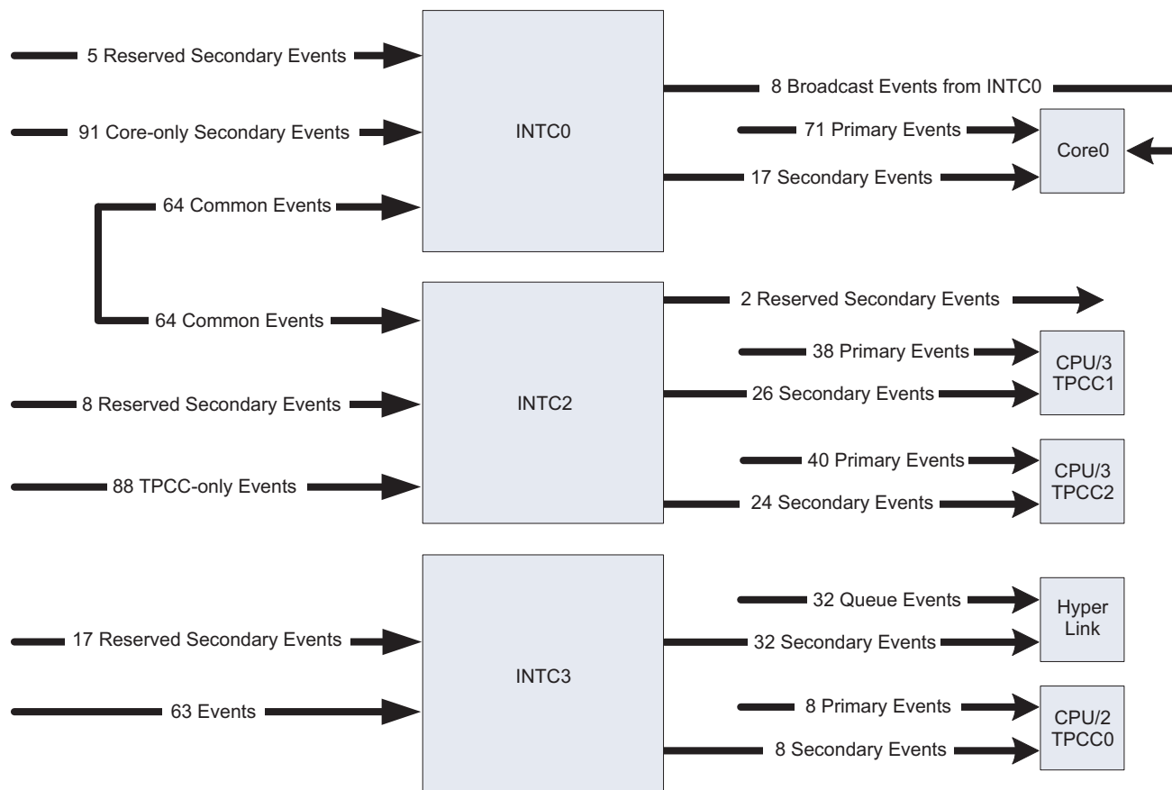
Figure 7-8 TMS320C6671 Interrupt Topology
