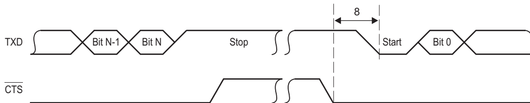
Figure 7-46 UART CTS (Clear-to-Send Input) — Autoflow Timing Waveform
