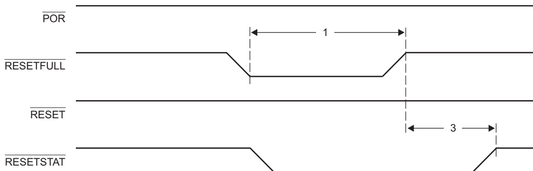
Figure 7-15 Soft/Hard-Reset Timing
