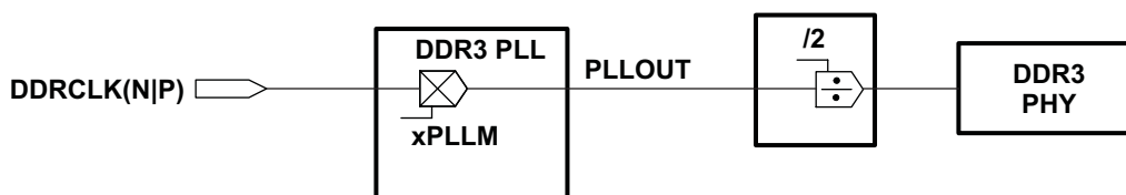
Figure 7-31 DDR3 PLL Block Diagram
