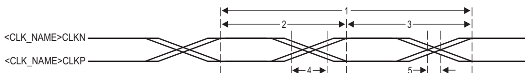
Figure 7-33 DDR3 PLL DDRCLK Timing
