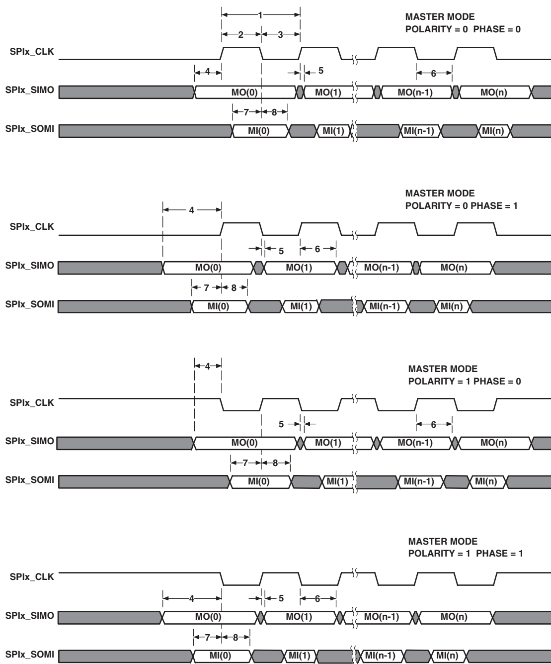
Figure 7-40 SPI Master Mode Timing Diagrams — Base Timings for 3 Pin Mode
