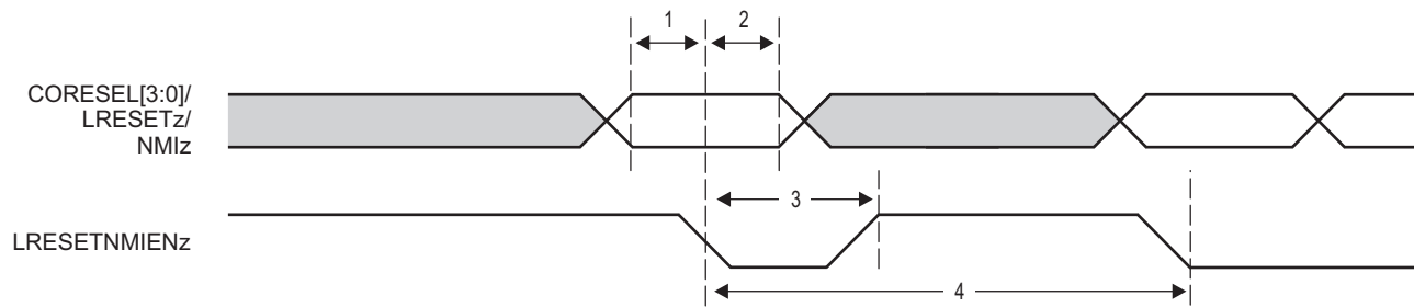
Figure 7-9 NMI and Local Reset Timing
