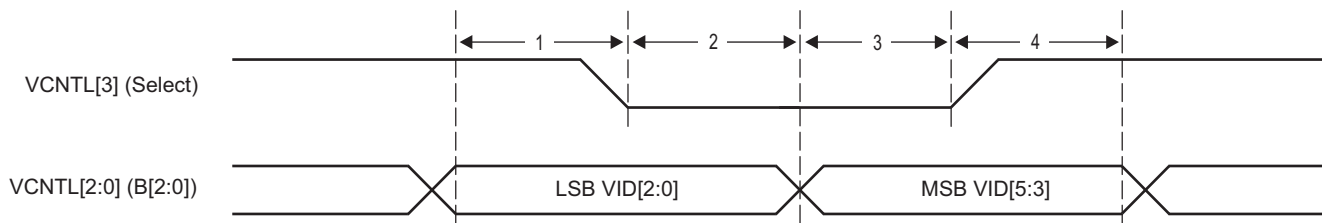
Figure 7-7 SmartReflex 4-Pin VID Interface Timing
